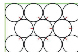
Pallet pattern
