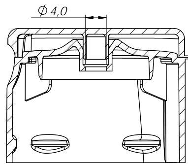
SECTION N-N
